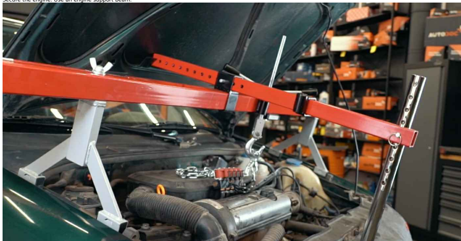
32 Unscrew the fastener of the cable bracket. Use a combination spanner #16.
