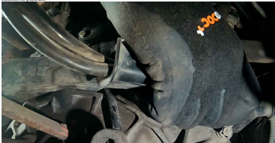
14 Unscrew the engine starter fasteners. Use a drive socket #13. Use a ratchet wrench.
