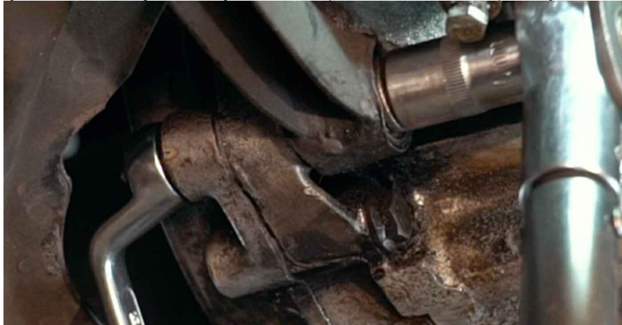
81 Tighten the fasteners that connect the gearbox to the engine block. Use a drive socket #18. Use a torque wrench. Tighten it to 64 Nm torque.
