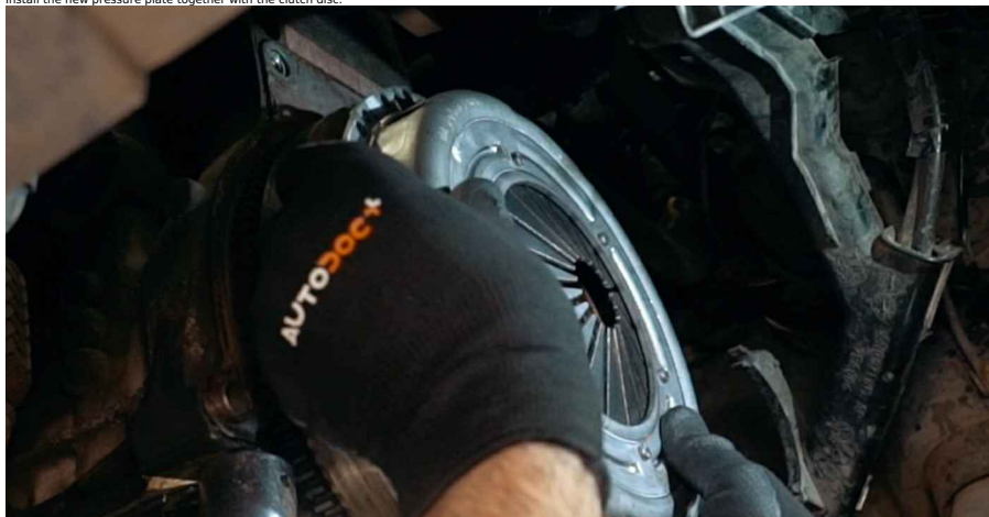
56 Screw in the pressure plate fasteners. Use 12-point socket No.9. Use a ratchet wrench.
