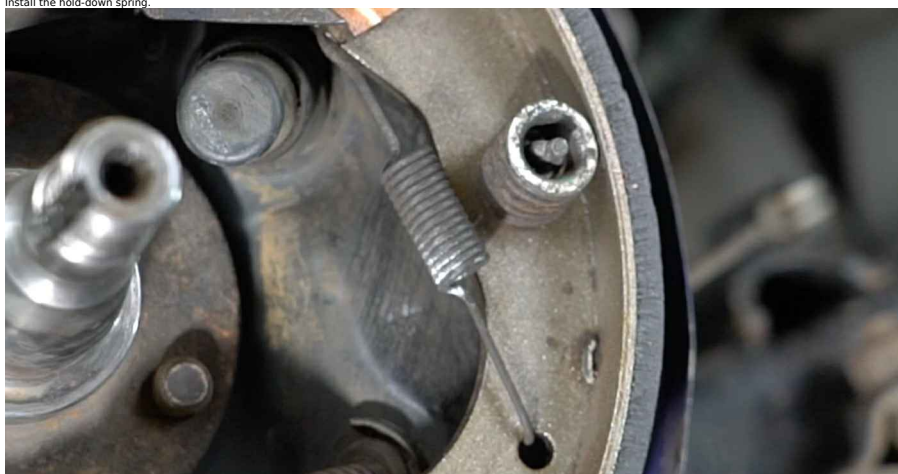
40 Install the upper return spring. Use long nose pliers.
